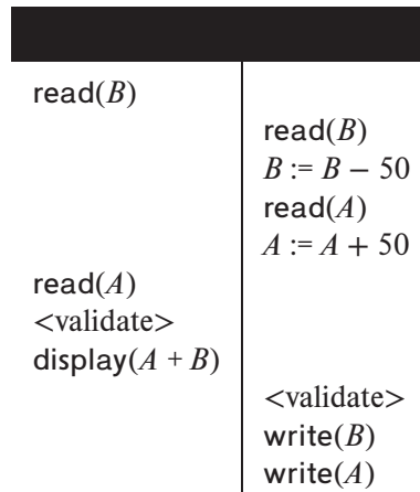
Figure 18.19 Schedule 6, a schedule produced by using validation.
