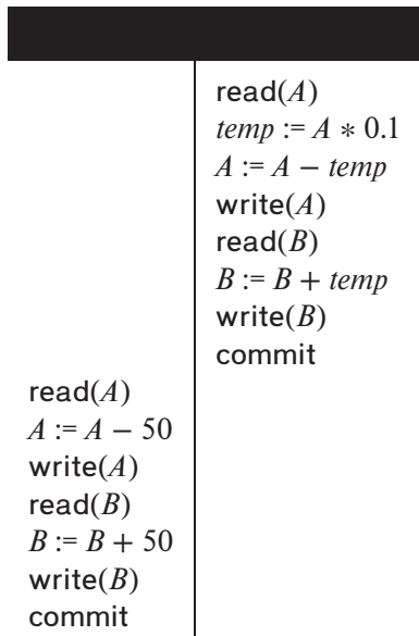
Figure 17.3 Schedule 2—a serial schedule in which T_2 is followed by T_1 .
