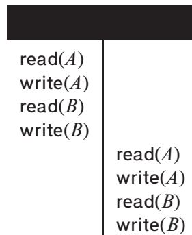
Figure 17.8 Schedule 6—a serial schedule that is equivalent to schedule 3.
