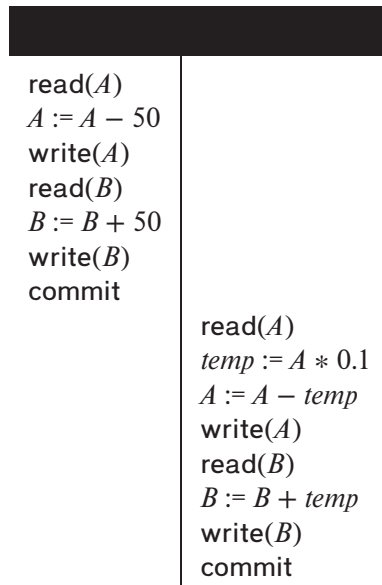
Figure 17.2 Schedule 1—a serial schedule in which T_1 is followed by T_2 .
