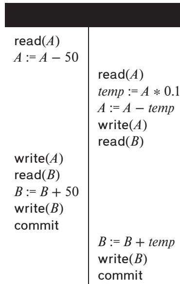
Figure 17.5 Schedule 4—a concurrent schedule resulting in an inconsistent state.
