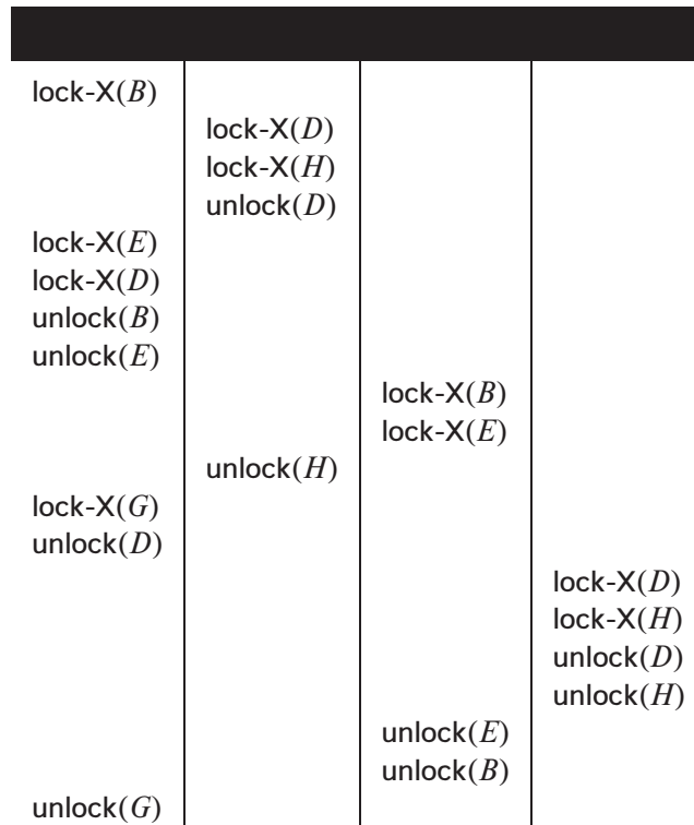
Figure 18.12 Serializable schedule under the tree protocol.
