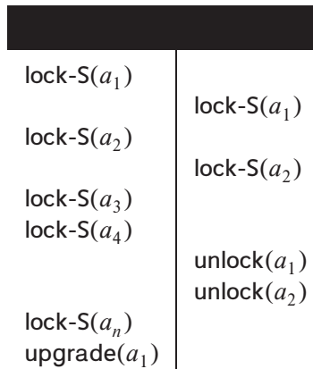
Figure 18.9 Incomplete schedule with a lock conversion.
