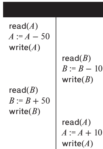
Figure 18.24 A non-conflict-serializable schedule.
