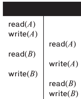
Figure 17.7 Schedule 5—schedule 3 after swapping of a pair of instructions.
