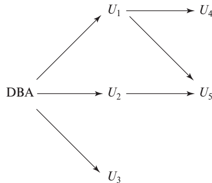
Figure 4.11 Authorization-grant graph ( U_1, U_2, \dots, U_5 are users and DBA refers to the database)
