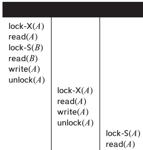
Figure 18.8 Partial schedule under two-phase locking.
