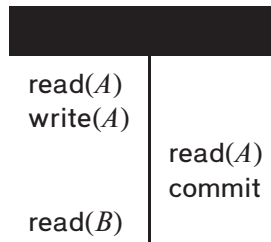
Figure 17.14 Schedule 9, a nonrecoverable schedule.
