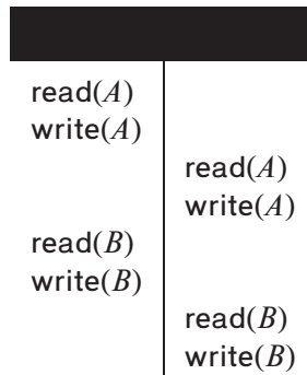
Figure 17.6 Schedule 3—showing only the read and write instructions.
