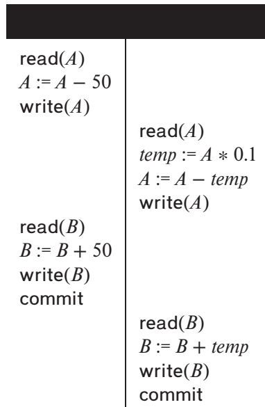
Figure 17.4 Schedule 3—a concurrent schedule equivalent to schedule 1.
