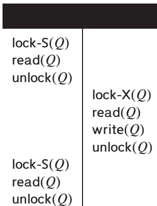
Figure 18.21 Nonserializable schedule with degree-two consistency.
