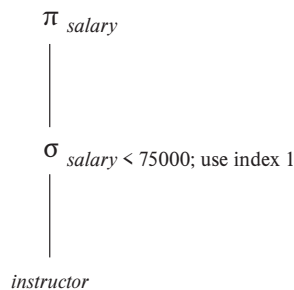
Figure 15.2 A query-evaluation plan.
