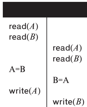
Figure 18.20 Nonserializable schedule under snapshot isolation.
