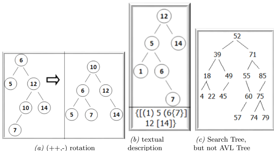
Figure 3. AVL Tree
