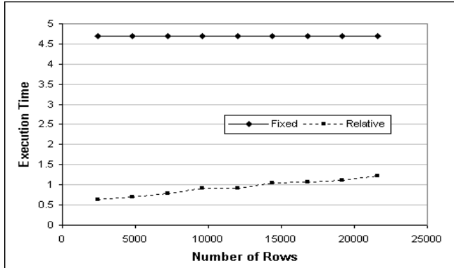
Figure 12 Pushing Predicates Optimization
