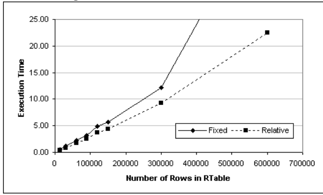
Figure 11 Fixed vs. Relative Translation
