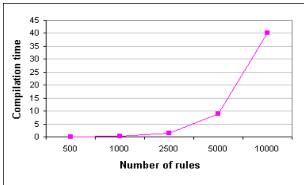
Figure 15 Collapsing of Rules.
