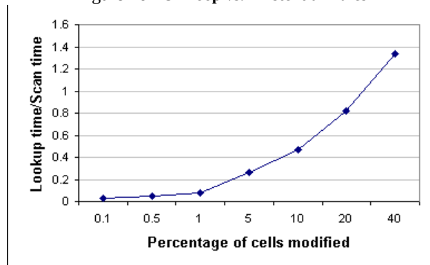
Figure 16 FOR loop vs. Existential Rules
