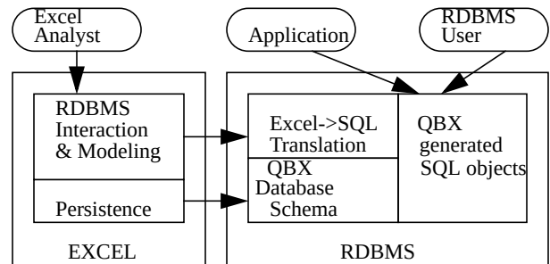
Figure 1 Architecture of QBX
