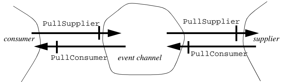
Figure 2-2 Pull-style communication between a supplier and an event channel and a consumer and the event channel
