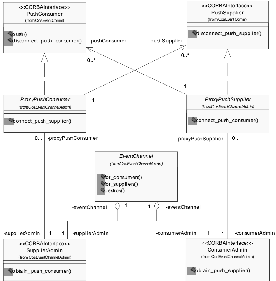
Figure 3-2 - Lightweight Event Service Interfaces and Classes
