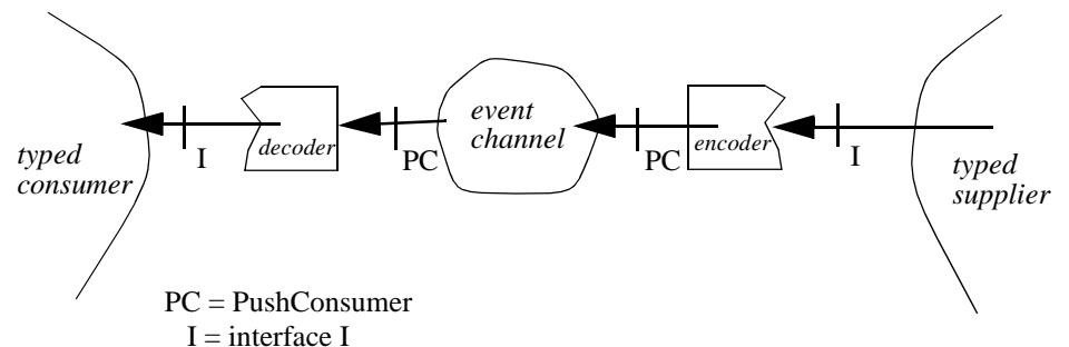
Figure A-1 A possible implementation of a typed event channel.
