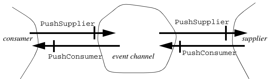
Figure 2-1 Push-style Communication Between a Supplier and an Event Channel, and a Consumer and an Event Channel
